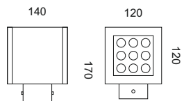
SW 9 UP*
