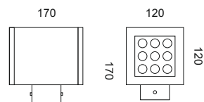
SW 9 UP&DOWN
